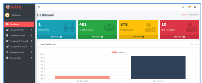
Figure 12. Dashboard Page
