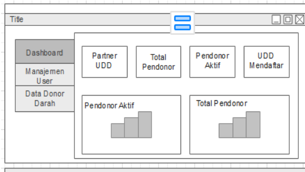
Figure 1. Mockup Dashboard
