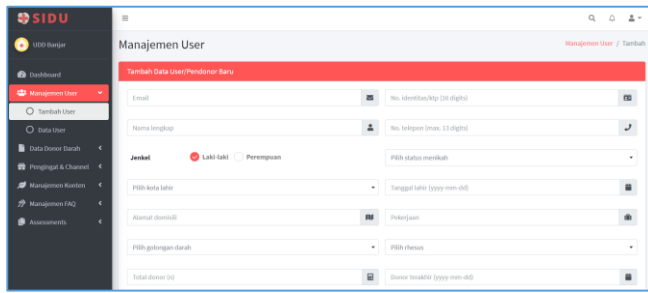
Figure 13. User Management
