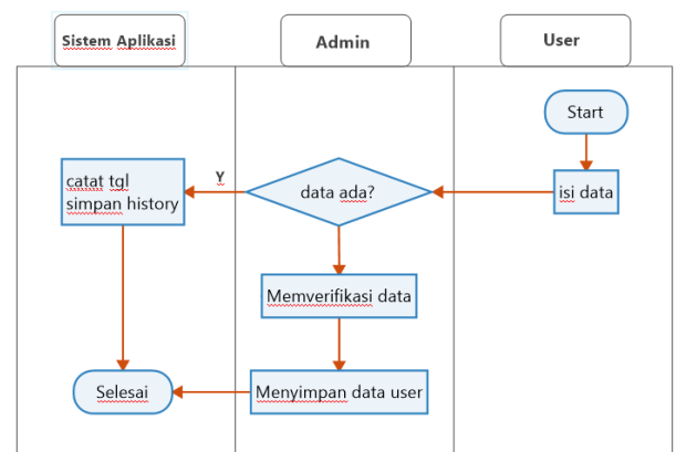
Figure 2. Activity Diagram: process for user input data
