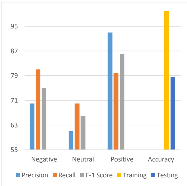
Figure 10. SGDC Report
