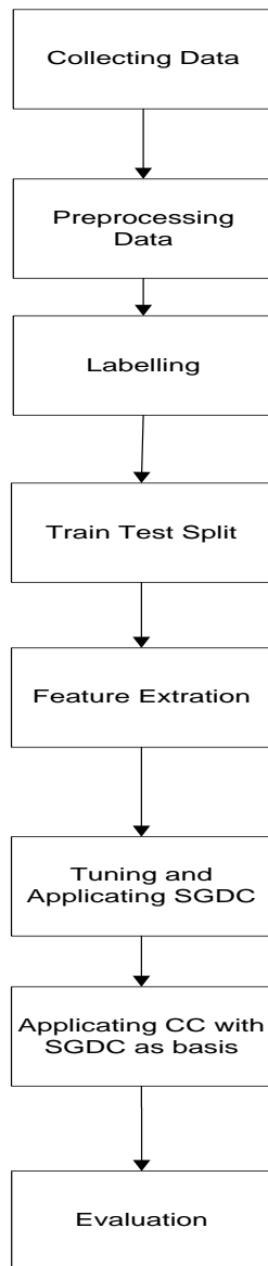
Figure 1. Research Method
