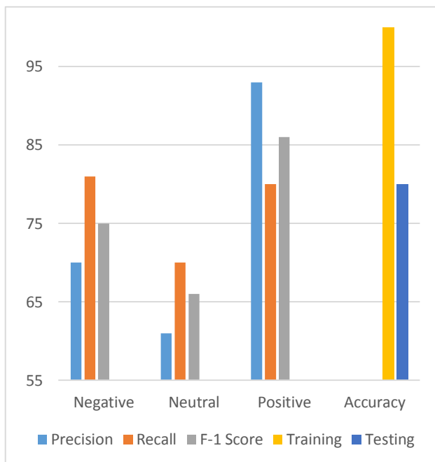
Figure 11. CC Report
