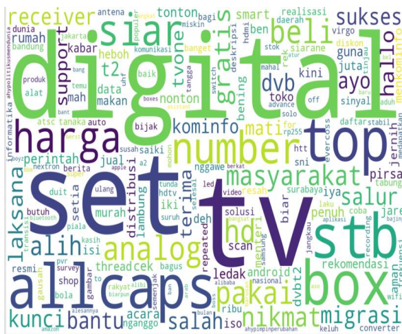
Figure 5. Neutral TF-IDF
