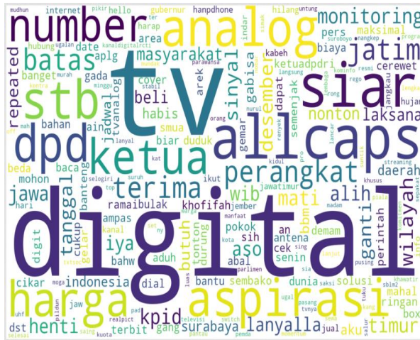
Figure 5. Neutral TF-IDF
