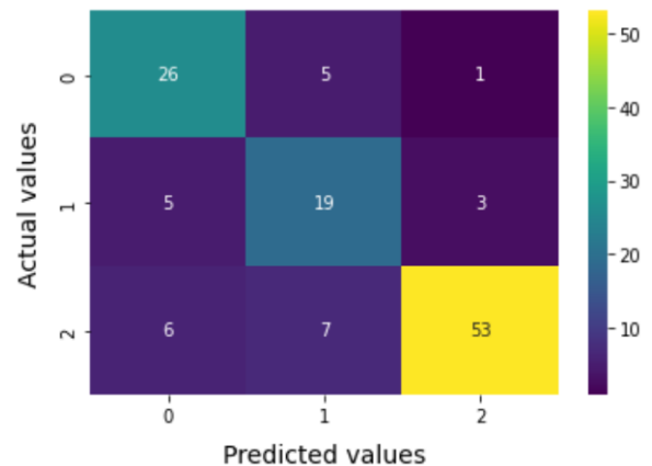
Figure 8. SGDC Evaluation
